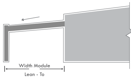
Lean - To
