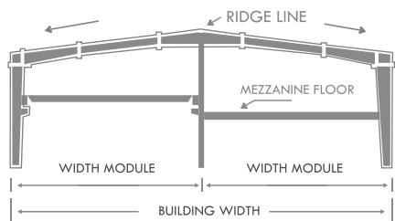
Multi Span I with Crane & Mezzanine
